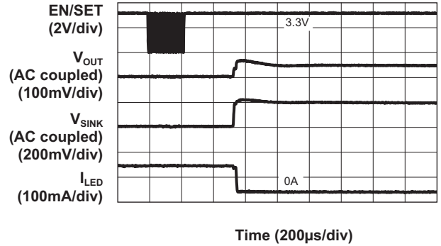
Movie Mode Current Transition (68.5mA/ch to 13.7mA/ch)
