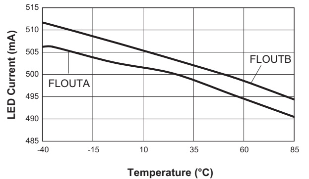
Flash Mode Current Matching vs. Temperature (500mA/ch)
